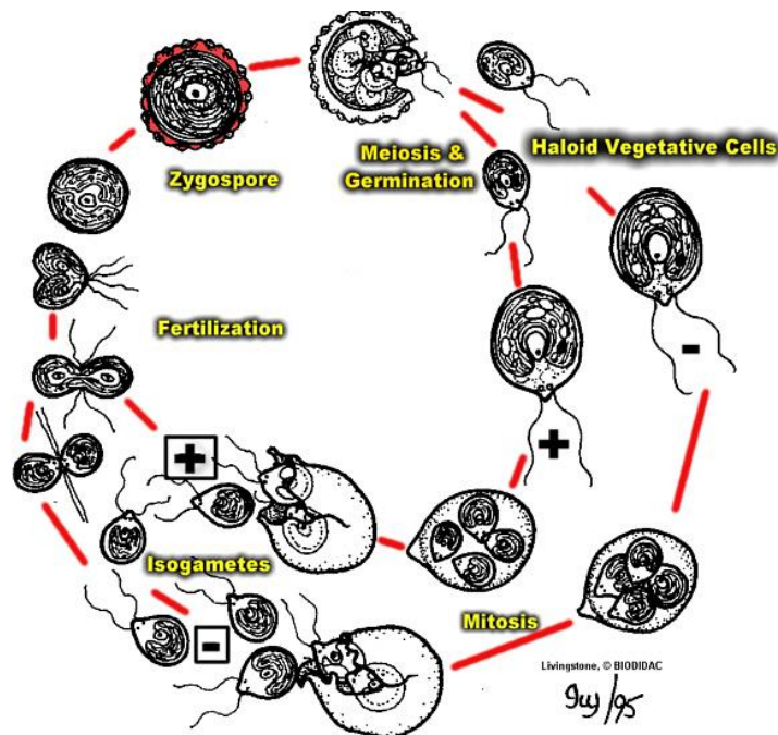
Figure 6. Chlamydomonas reproduction
