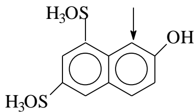
2-Naphthol-8-sulphonic acid
