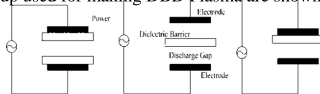
Figure.4 Three basic configurations
