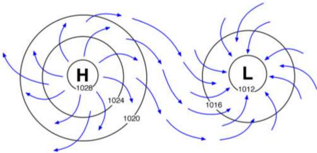
A high pressure and a low pressure center with wind directions (northern hemisphere). Circles are isobars with pressure in mb.
