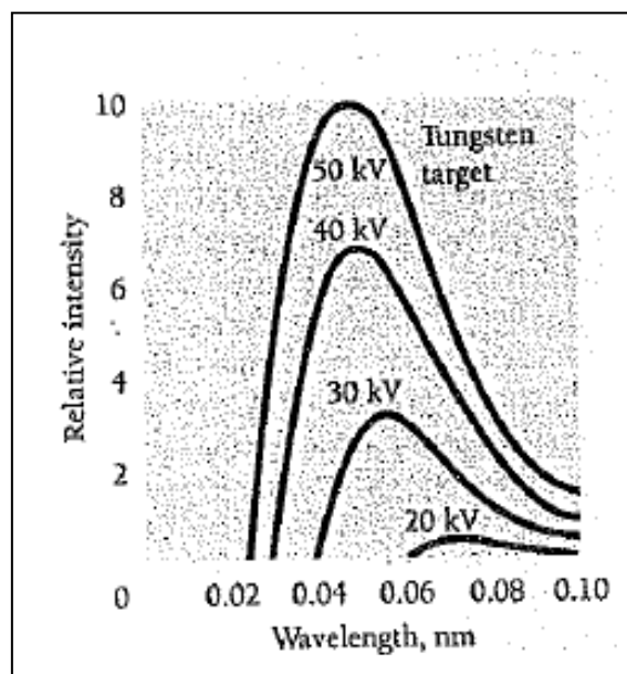
Figure X-ray spectra of tungsten at various accelerating potentials
