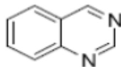
quinazoline
