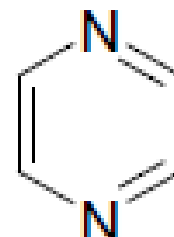
Pyrazine
