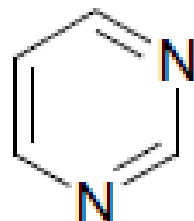
Pyrimidine
