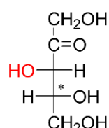
D-Xylulose
