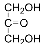
Dihydroxy acetone
