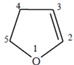
\Delta^2 -Oxolene
