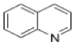
quinoline
