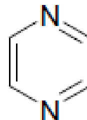
Pyrazine
