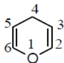
4H -Oxin
