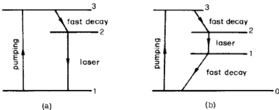
FIG. 1.4. (a) Three-level and (b) four-level laser schemes.
