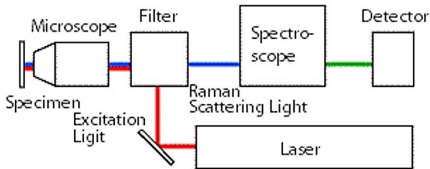
▲ Components of Raman Microscope
