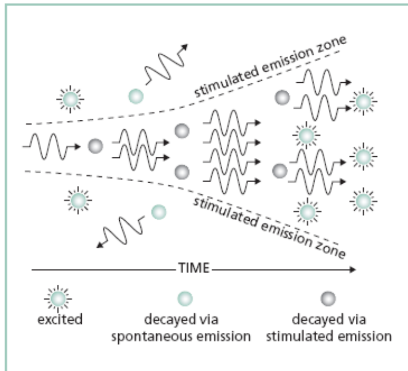
Figure 36.3 Amplification by stimulated emission
