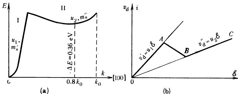
Figure 6.17 The Gunn effect: (a)—structure of conduction band in gallium arsenide in [100] direction; (b)—variation of drift velocity and current density with the increase in electric field intensity.
