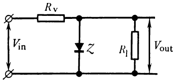
Figure 8.20 Circuit diagram of the simplest voltage regulator using a silicon Zener diode Z .
