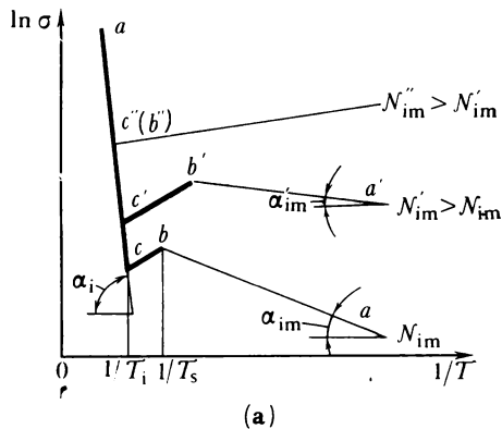
Figure 6.14 Temperature dependence of specific conductance of impurity semiconductors: (a)—theoretical curve; (b)—experimental plots for silicon containing different amounts of phosphorus.
