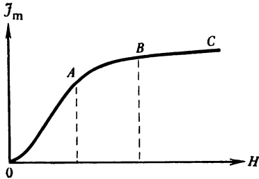
Figure 7.21 Magnetization plot of a ferromagnetic: OA —section corresponding to the process of displacement of domain boundaries, AB —section corresponding to rotation of magnetization vector, and BC —section corresponding to the paraprocess.
