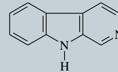
carboline
