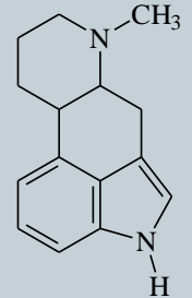
indole + hydroquinoline
