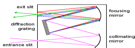
Monochromator
