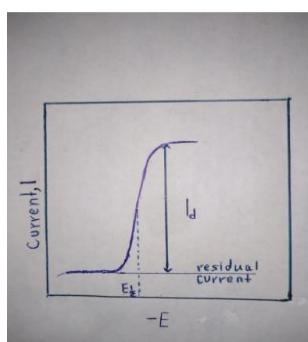
The polarogram
