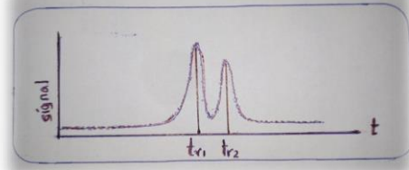
The chromatogram
