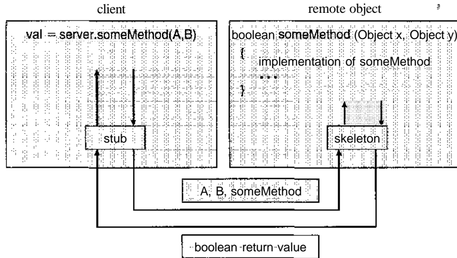
Figure 3.23 Marshalling parameters.
