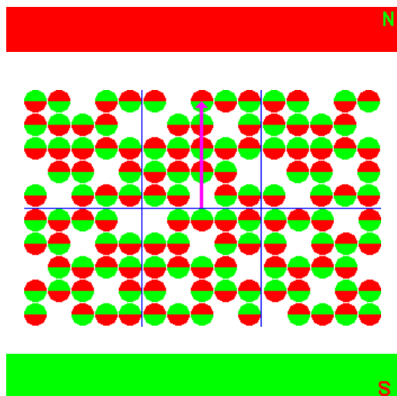
Figure 44 net magnetization
