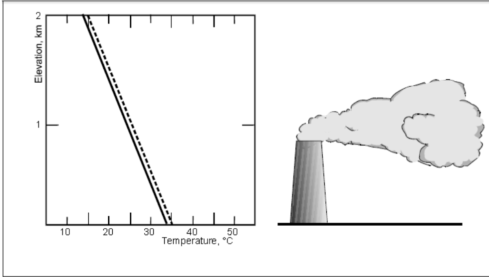
Coning plume
