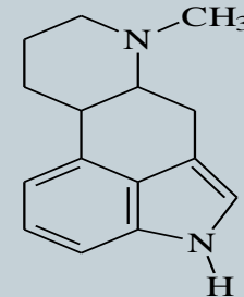
indole + hydroquinoline
