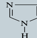
imidazole
