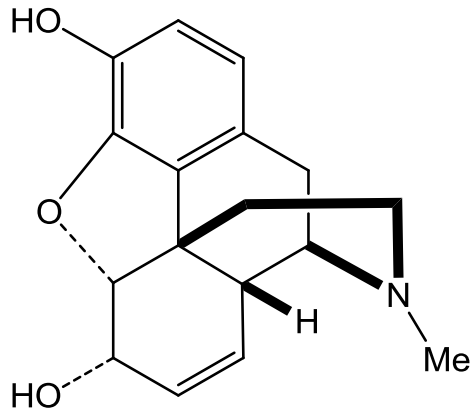
Morphine
