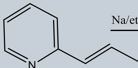
2-propenyl pyridine
