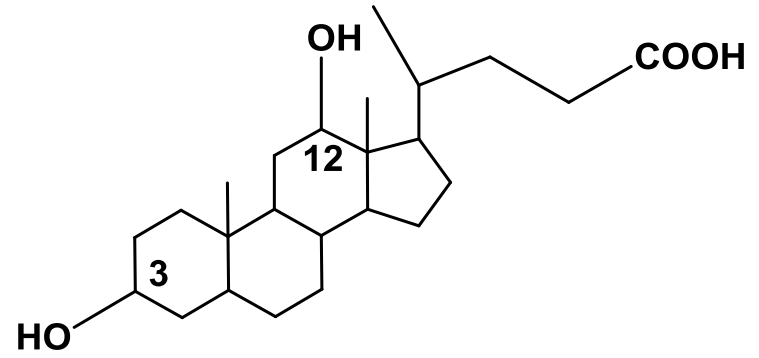
3,12-dihydroxycholanic acid
