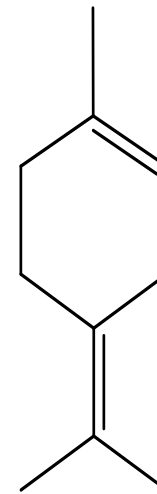
P-meth-1,4(8)diene
