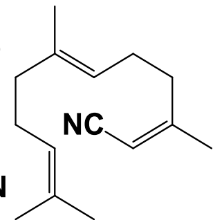
farnesal cyanide (4)
