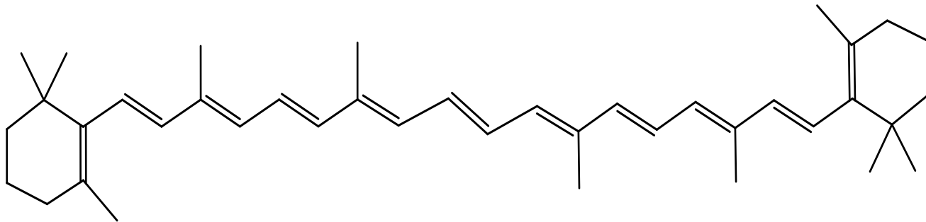
B - Carotene
