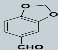
Piperonal
