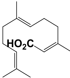
Farnesenic acid (5)
