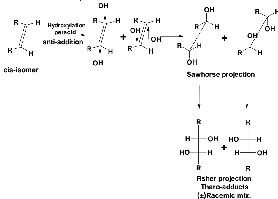
Scheme 7.6
