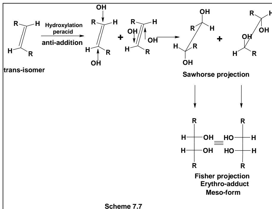
Scheme 7.7
