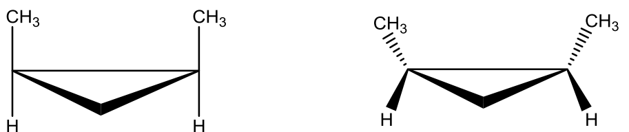
cis -1,2-dimethylcyclopropane
