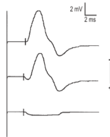
FIGURE 2-19 Volume conduction and motor potentials. With the active recording electrode (G1) over the motor point, depolarization first occurs at that site, with the depolarization subsequently spreading away. The corresponding waveform has an initial negative deflection without any initial positivity (top trace). If the active recording electrode is off the motor point, depolarization begins distally and then travels under and past the active electrode, resulting in an initial positive deflection (middle trace). If the depolarization occurs at a distance and never travels under the recording electrode, only a small positive potential will be seen (bottom trace). Note that, by convention, negative is up and positive is down in all nerve conduction and electromyographic traces.
