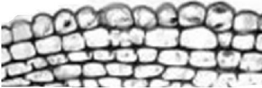
normal epidermis
